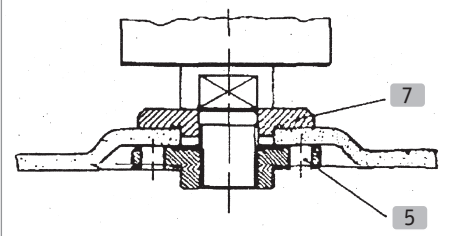
3 Flange arrangement for depressed centre cutting discs
